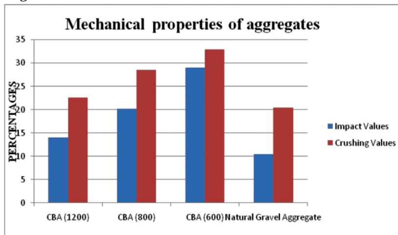
Figure 1: Mechanical Properties of Aggregates
