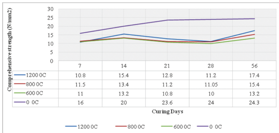
Figure 2: Compressive strength of concrete cubes produced with clay aggregates exposed to 600°C, 800°C and 1200°C
