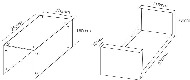
Figure 10: Inverter casing
