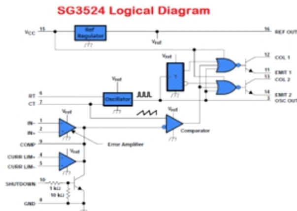
Figure 6: The Internal Circuit of SG3524
