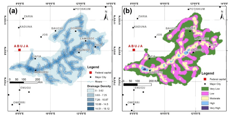
Figure 9: (a) Drainage Density and (b) Reclass Drainage Density
